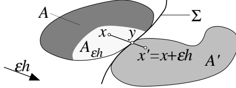
FIG.1. The set A_{\varepsilon h} for given \varepsilon > 0 and h \in \mathbb{R}^N .
