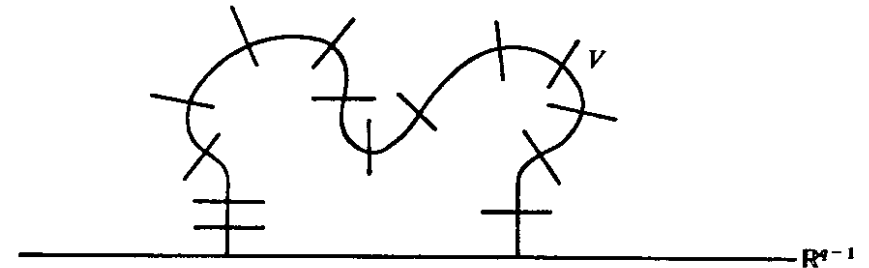
Figure 4-3. A normal tubular neighborhood of V in \mathbb{R}_+^q .
