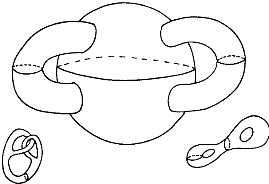
Figure 1-5. Orientable surfaces of genus p = 2 .
